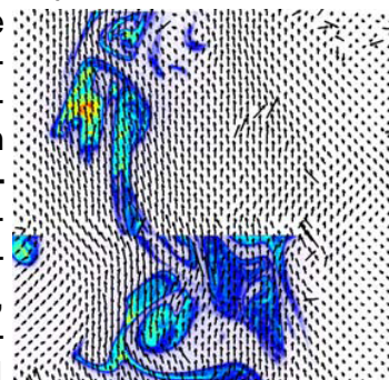
Simultaneous LII and PIV soot ↔ flow field
